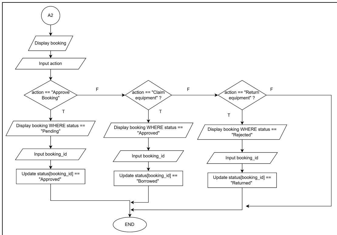
Figure 5: Admin Booking Flowchart
