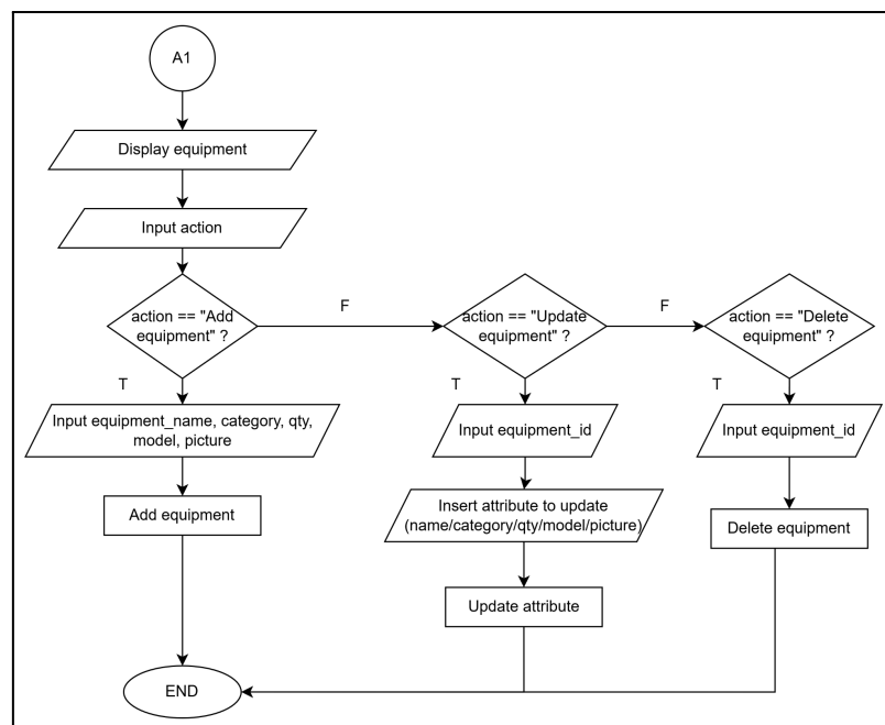
Figure 4: Admin Equipment Flowchart
