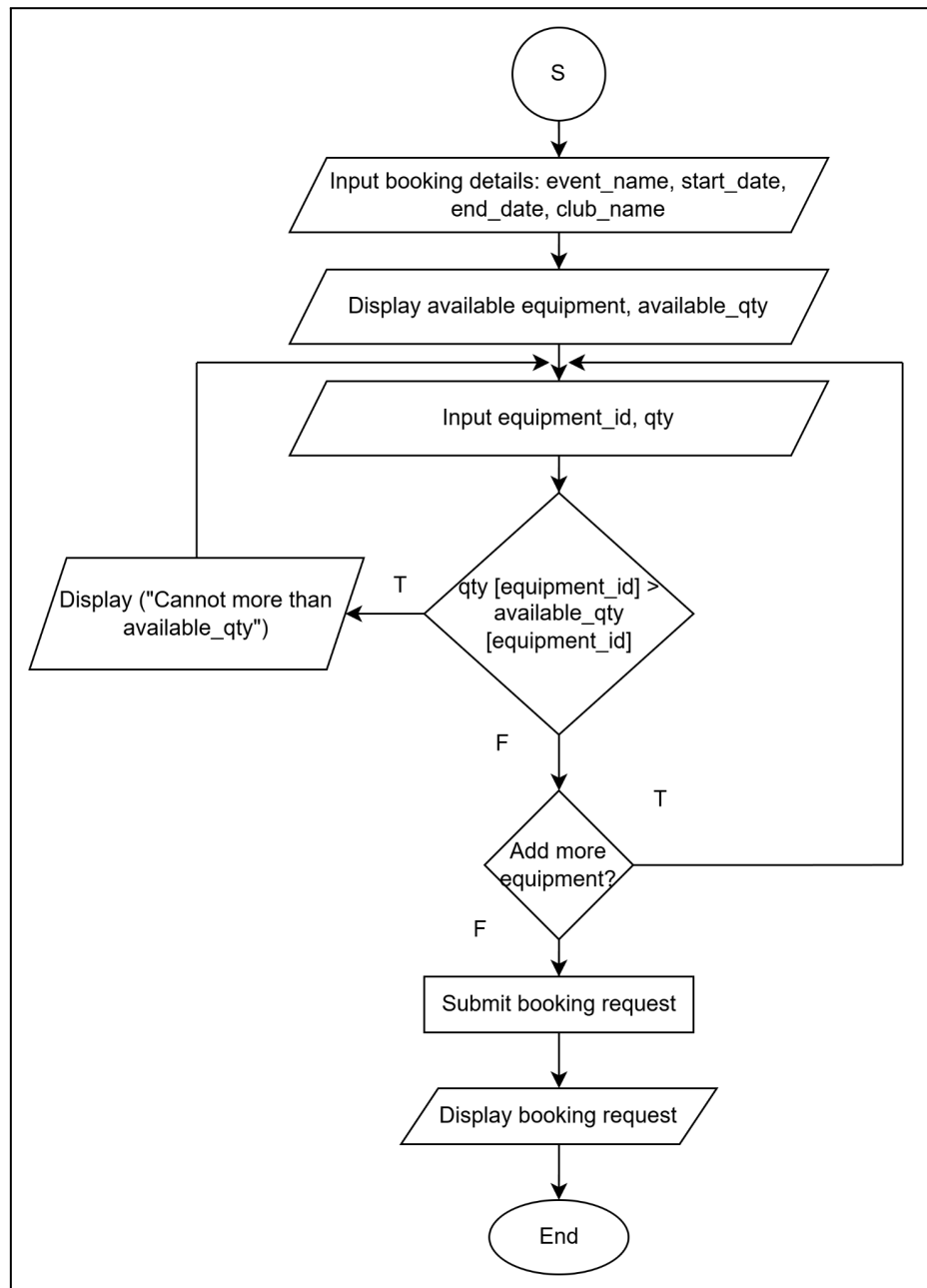
Figure 2: User Flowchart
