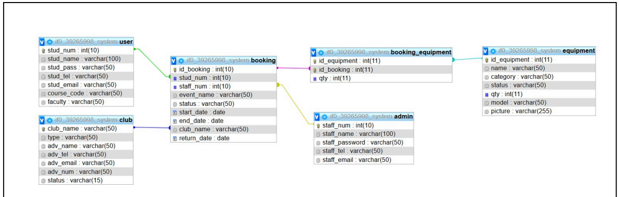
Figure 6: ERD
