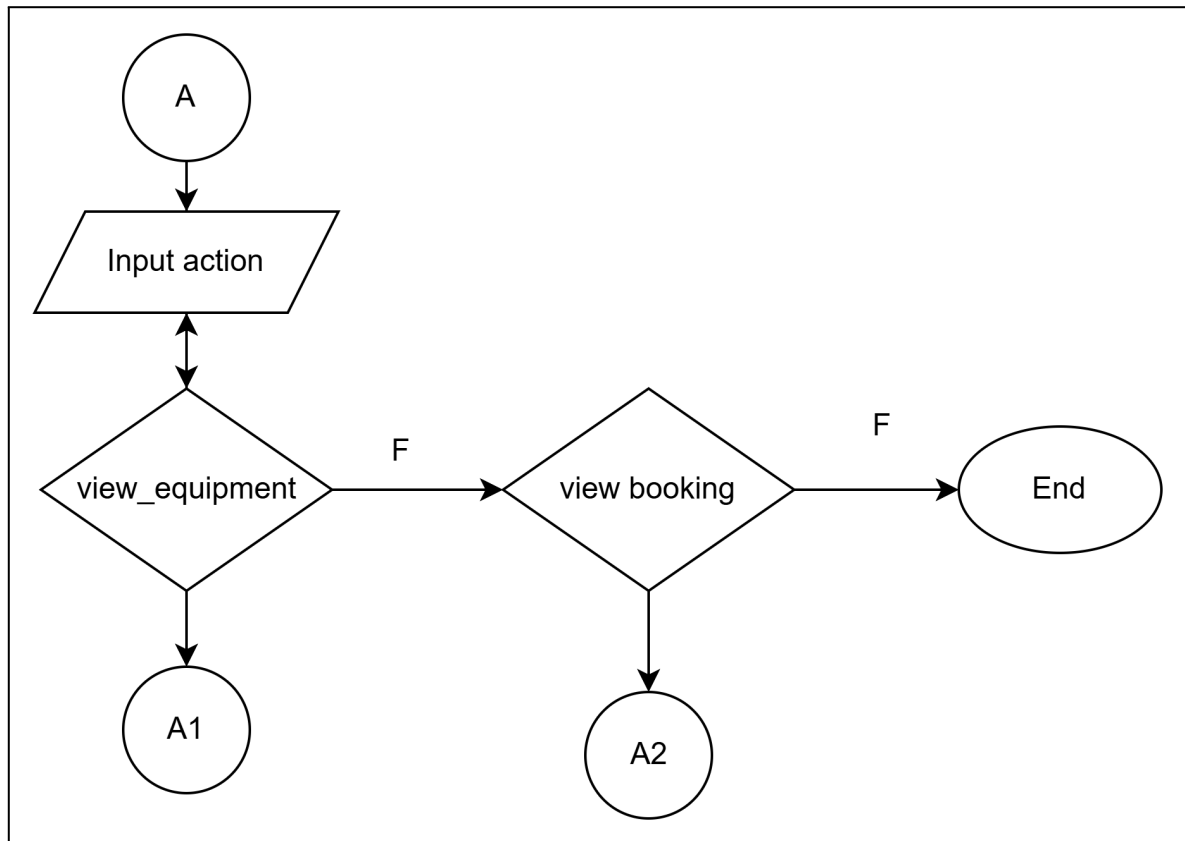
Figure 3: Admin Flowchart
